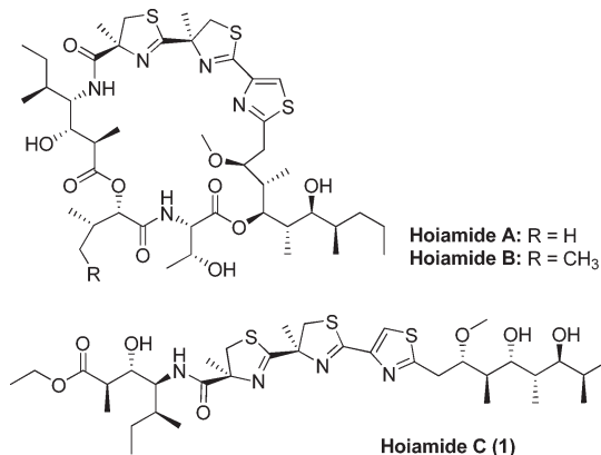
Figure 1. Structures of hoiamides A–C.
