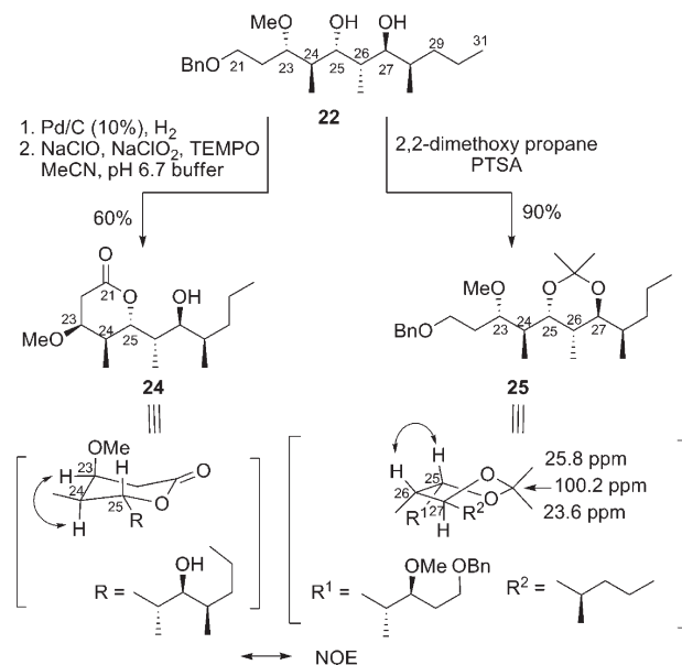
Scheme 5. Assignment of Stereochemistry of 22
