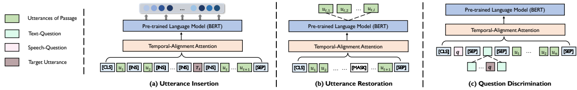
Figure 2: Auxiliary tasks in Self-supervised training.
