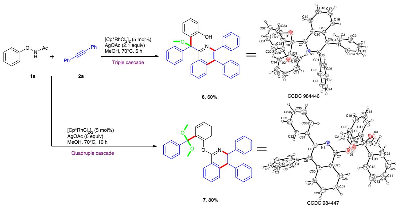
Figure 3 | Multistep cascade reactions. Conditions for 6 : N -phenoxyamide (0.2 mmol), diphenylacetylene (0.44 mmol), [\text{RhCp}^*\text{Cl}_2]_2 (5 mol%), \text{AgOAc} (2.1 equiv.), \text{MeOH} (1 ml), isolated yield. Conditions for 7 : N -phenoxyamide (0.2 mmol), diphenylacetylene (0.44 mmol), [\text{RhCp}^*\text{Cl}_2]_2 (5 mol%), \text{AgOAc} (6 equiv.), \text{MeOH} (1 ml), isolated yield.
